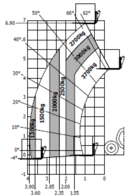
MLT 737 130 PS+
